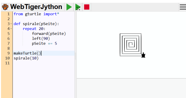
Python
